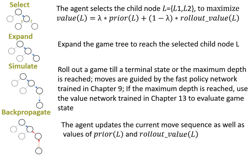
Figure 16.1 Steps of tree search when implementing the AlphaGo algorithm in the coin game
